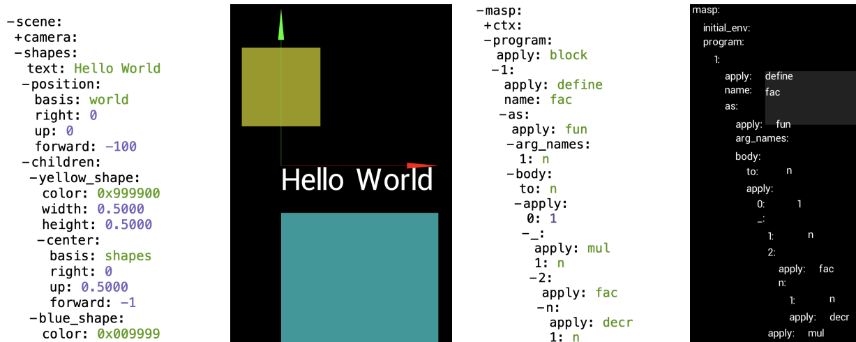
Figure 6 Memory-mapped display mechanism in BootstrapLab. A sample scene consisting of text, rectangles and arrows (a) with rendering (b). A tree representing a MASP function, rendered outside of BootstrapLab (c) and using the memory-mapped display mechanism (d). Image source [40].
