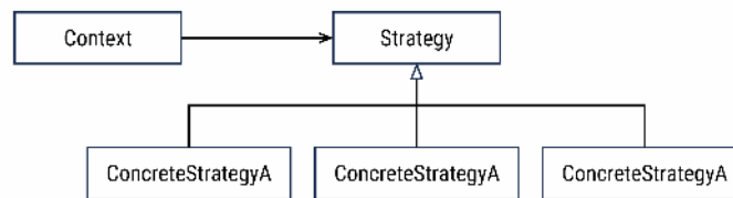
Figure 7: A class diagram illustrating the relationships between classes and interfaces in the case of the Strategy design pattern. The Context class uses a Strategy to do some work and there is a number of specific strategies that can be supplied to it.
